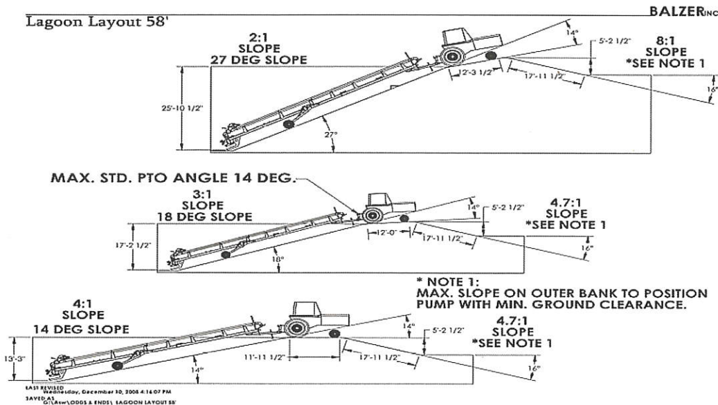
Trailer Mount Prop Agitator
